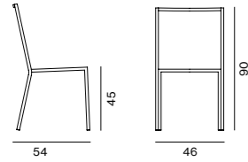
Chair / Sedia / Chaise / Stuhl
